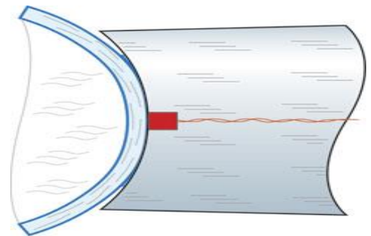
Fig 12: Principle of Contour Matching and the sensor in Pascal DCT
