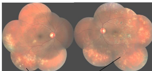
Multifocal Choroiditis
