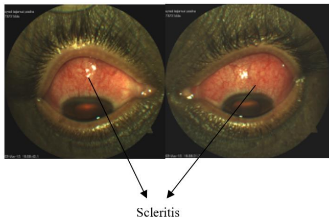
Figure 1: Tubercular scleritis
